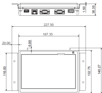
PFXGP4402WADWR(带安装托架)
